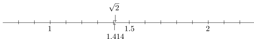
Figure 1.2: APPROXIMATING \sqrt{2} WITH RATIONAL NUMBERS.
